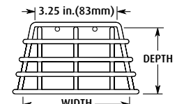
STI-9620 END VIEW
