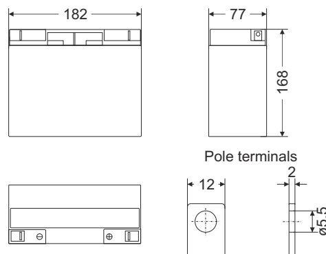
Dimensions [mm] Tolerance: +/- 2mm;
