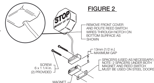
VIEW SHOWING MAGNET INSTALLATION NB: FITTING UNIT AWAY FROM DOOR (OPTIONAL)
