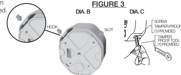
VIEW SHOWING HOW TO FIX THE COVER TO THE BASE
