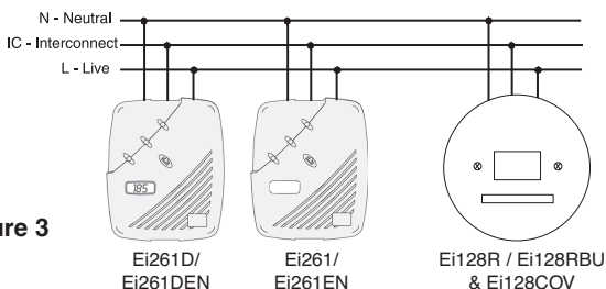
The above shows the connection for Carbon Monoxide Alarms. Connect the Smoke/Heat Alarm similarly but on a separate circuit to the Carbon Monoxide Alarm (unless an Ei159 Locator Switch is used on the system)
